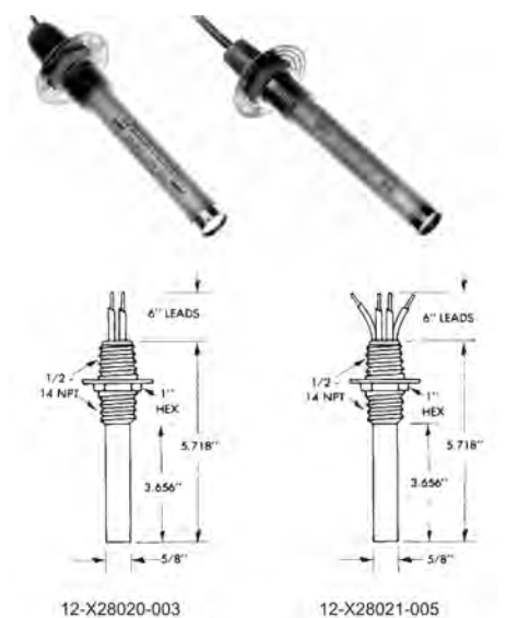
Figure 5. Coupling Head
