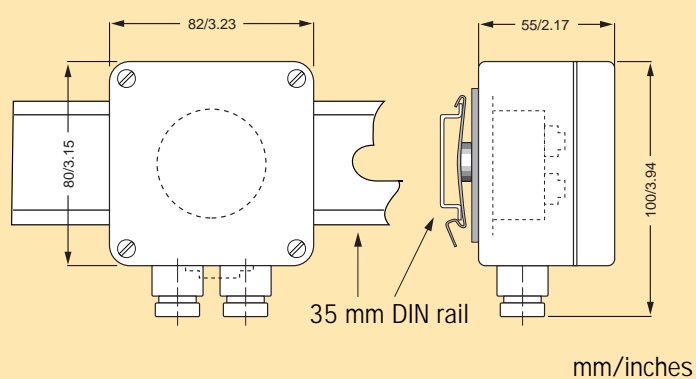
Field box for DIN rail mounting
