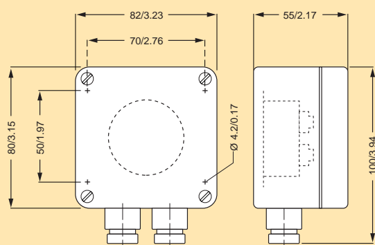
Field box for surface mounting
