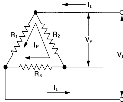
Delta Wiring Configuration
