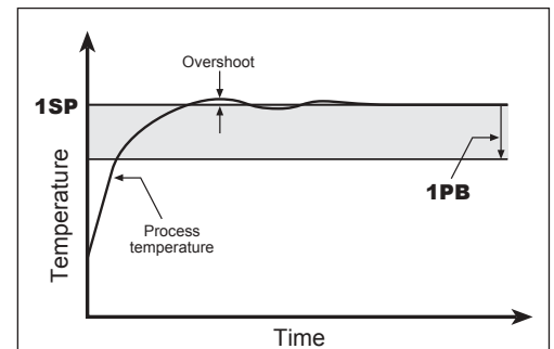
Figure 5 Proportional-Integral-Derivative Control (PID) in heating mode
